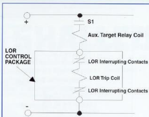
Figure 7 - LOR Control Circuit w/Aux. Target
