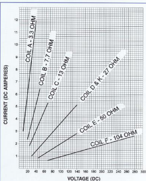
Figure 5 - Trip Solenoid Coil Data.
