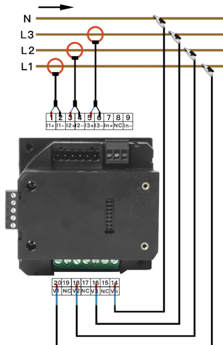
Figure 3-2 3P4W_3CT
