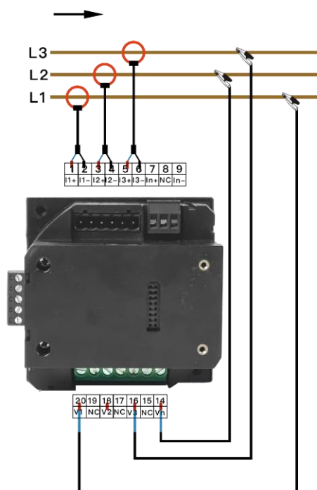
Figure 3-3 3P3W_3CT
