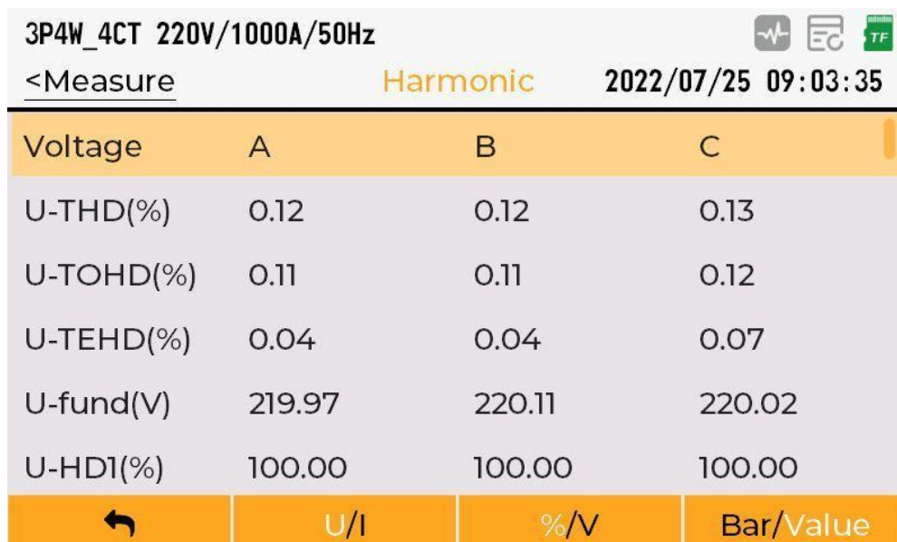
Figure 5-38 Harmonic value display
