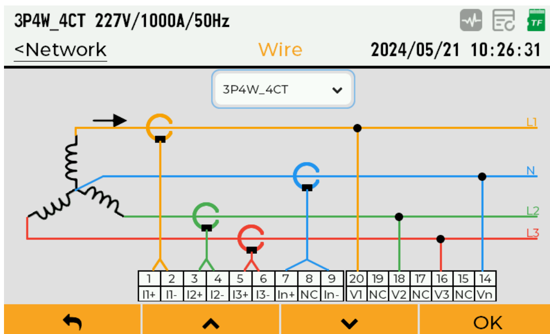
Figure 5-5 Wiring mode configuration
