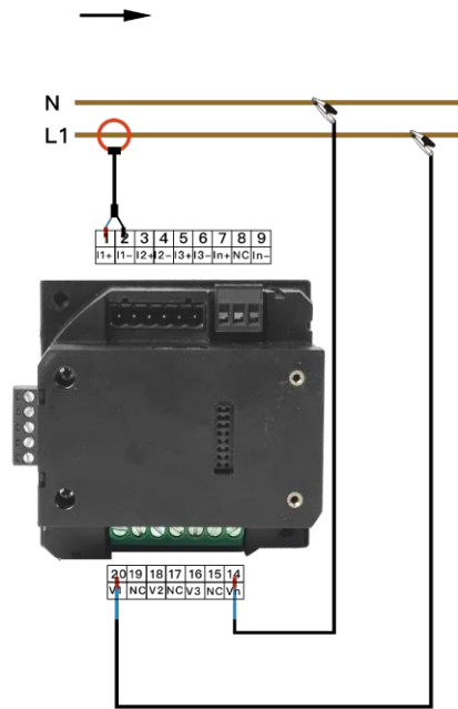
Figure 3-6 1P2W
