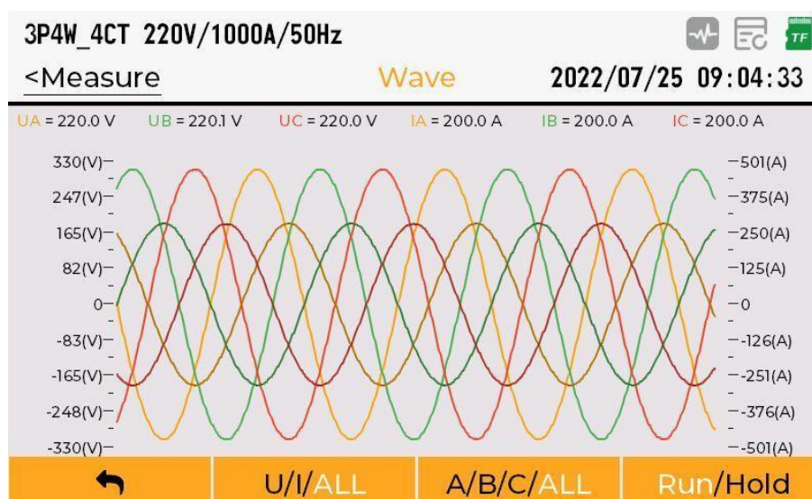
Figure 5-39 Voltage and current waveform display
