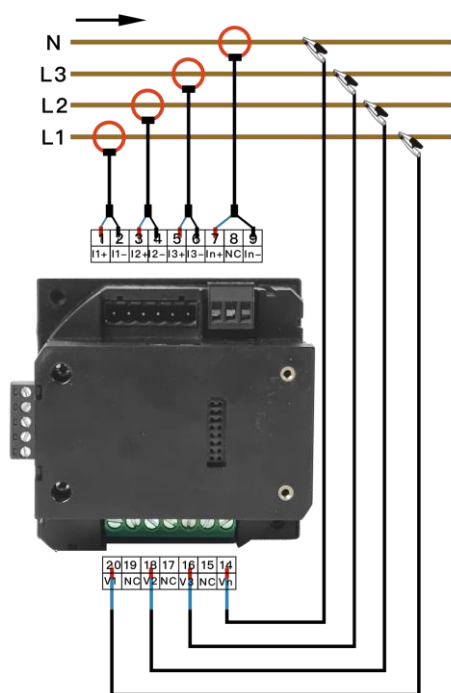
Figure 3-1 3P4W_4CT
