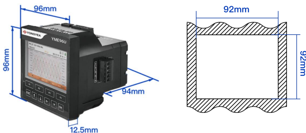
Figure 2-1 Product appearance
