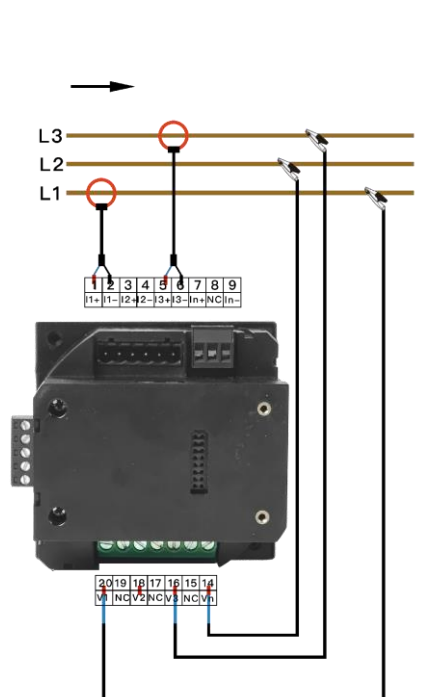
Figure 3-4 3P3W_2CT
