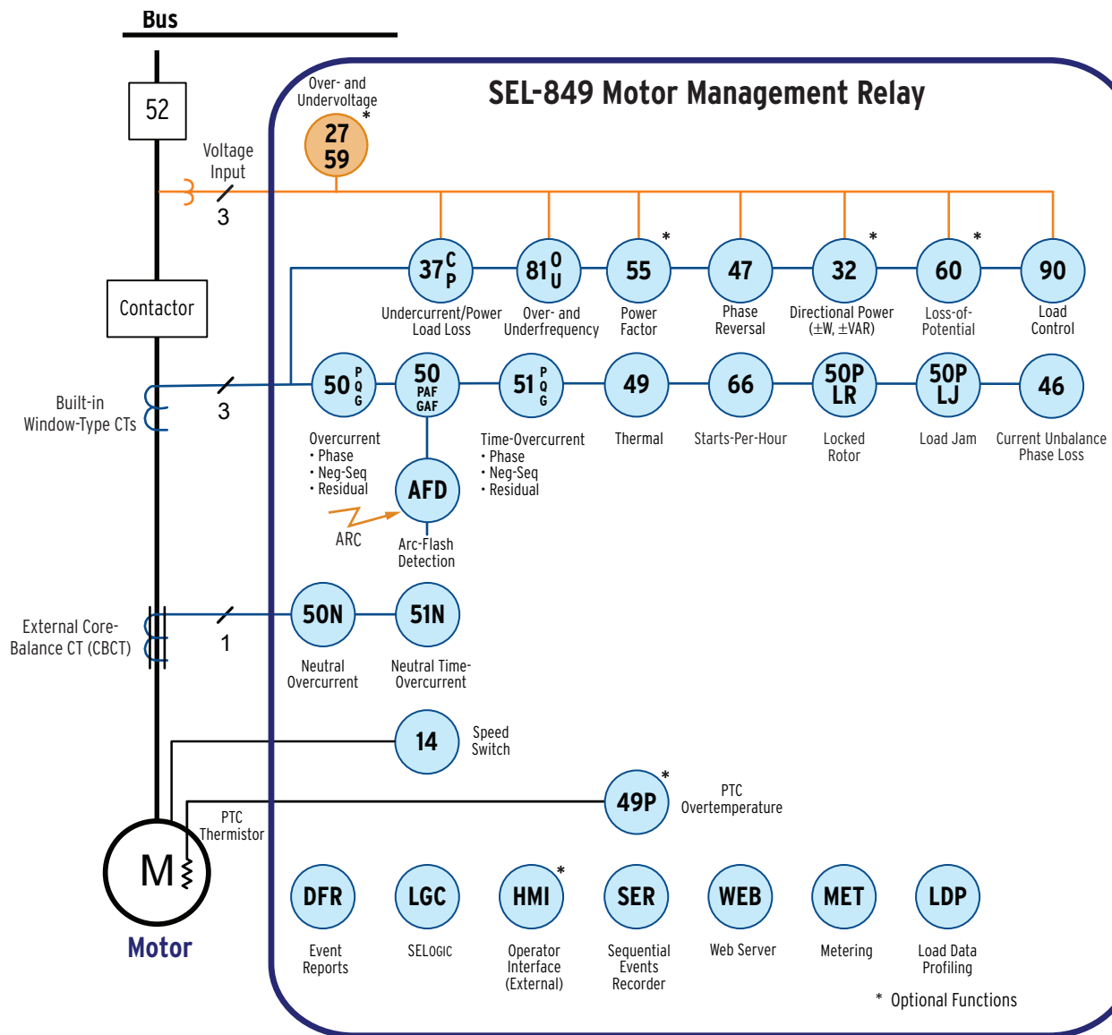
Figure 1 Functional Diagram
