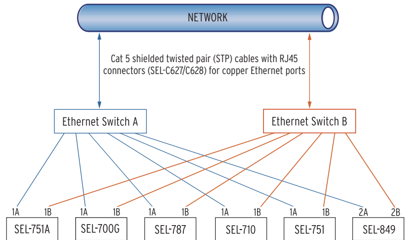
Figure 4 Simple Ethernet Network Configuration With Dual Redundant Connections (Failover Mode)
