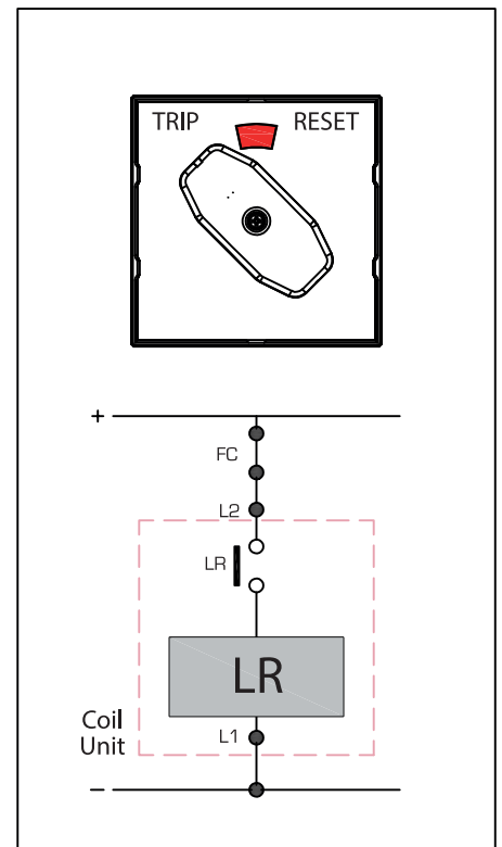
FAULT CONDITION Handle Spring return in TRIP position Contact LR open and contact FC close won't possible restore the LOR in RESET position until the contact FC will be close.
