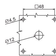
PANEL DRILLING F1.013
