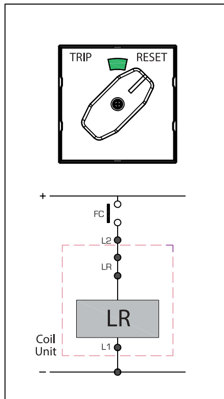
NO FAULT CONDITION Handle in RESET position Contact LR closed and contact FC open.
