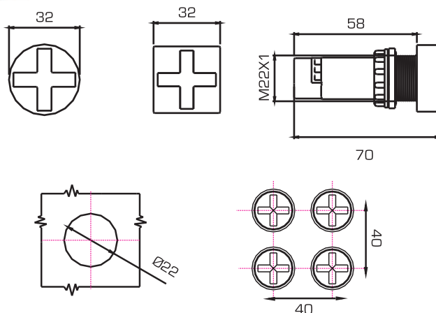
PANEL DRILLING
