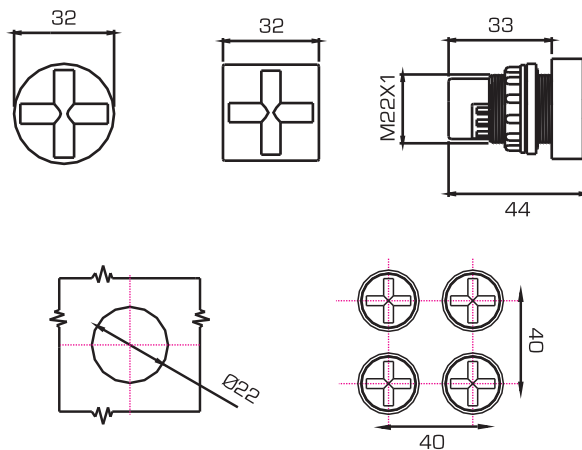
PANEL DRILLING
