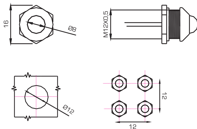
PANEL DRILLING
